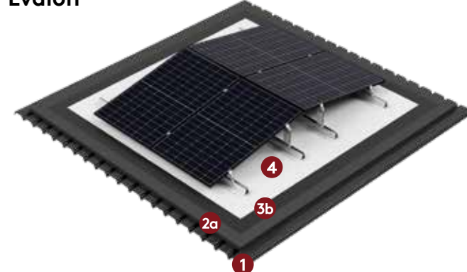
Roof-Solar Evalon®
